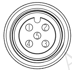
Conn. 1 & Conn. 2 Pin Assignments Front View
