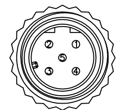
Conn. 1&2 Pin Assignments Front View
