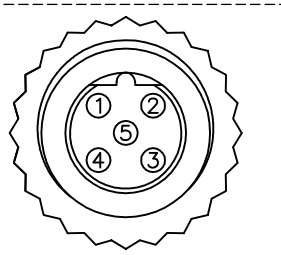
Conn.1&2 Pin Assignments Front View
