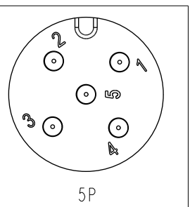
5P Pin Assignments Front View
