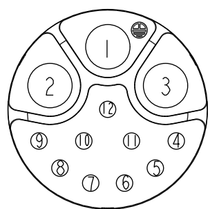
CI & C2 Pin Assignments Front View
