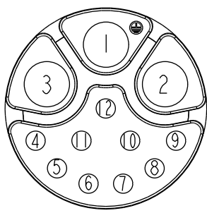
C1 Pin Assignments Front View
