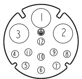
C1 Pin Assignments Front View
