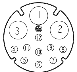
C2 Pin Assignments Front View
